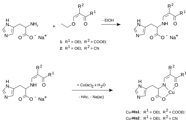
Scheme 2 Synthesis of formally tricoordinated copper(II) complexes, derived from 3-oxo-1-enamines of histidine. The imidazole NH is arbitrarily localized at the δ-N as in the cyclic oligomers of the complexes.
