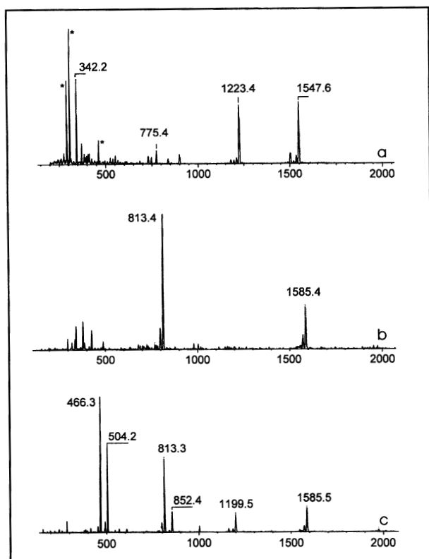
Fig. 4 Mass spectra of Cu-His1: a) FAB technique with nitrobenzylalcohol (nba), *signals of nba; b) ESI technique ( \text{HCCl}_3/\text{MeOH} ); c) ESI technique (pyridine).
