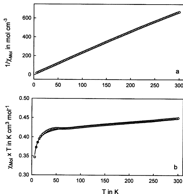
Fig. 5 Magnetic susceptibility of solvent free Cu-His1: a) reverse molar susceptibility plotted versus temperature. b) \chi_M \times T plotted versus temperature. The solid line is calculated from a fit of the data to the Curie-Weiss expression considering the temperature independent paramagnetism (TIP).
